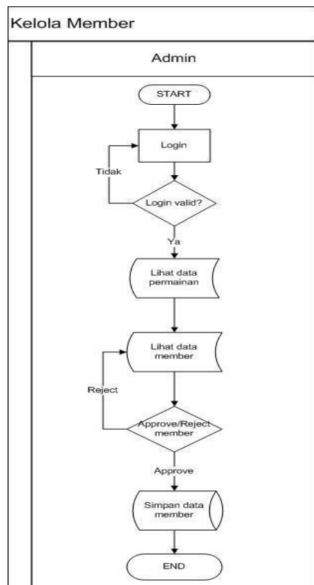
Gambar 2 Flowmap Kelola Member
