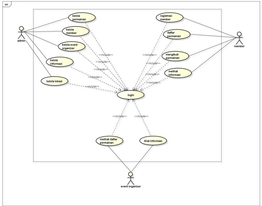
Gambar 12 UseCase Diagram
