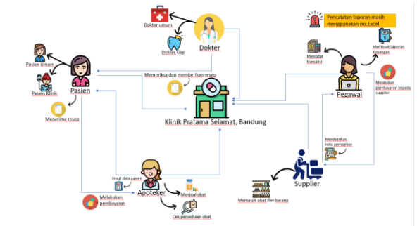
Gambar 3- 2 Rich Picture
