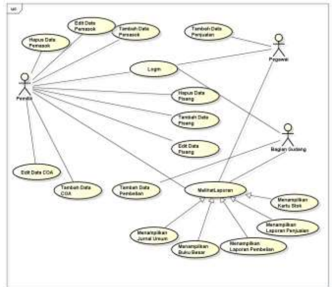
Gambar 1 Usecase Diagram
