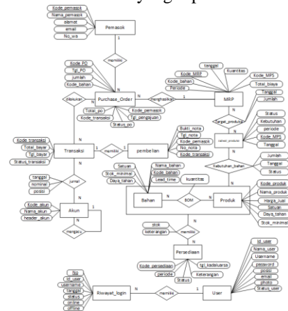
Gambar 3 - 2 Entity Relationship Diagram
