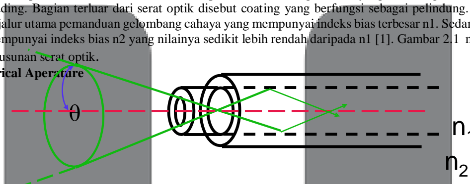
Gambar 2.2 Numerical Aperature
