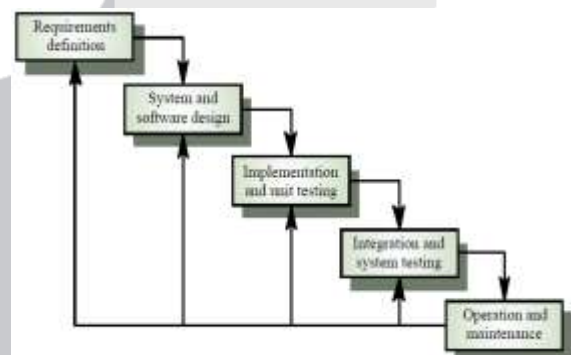
Gambar 1 Model Waterfall [1]
