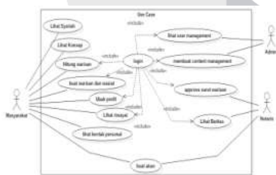
Gambar 2 Usecase
