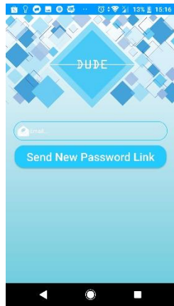
Gambar 4.12 Reset Password
