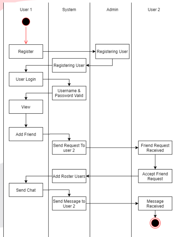
Gambar 3.2 Activity Diagram
