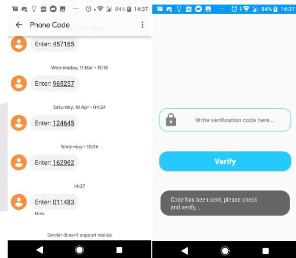
Gambar 4.4 OTP
