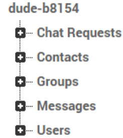
Gambar 3.8 Folder Database
