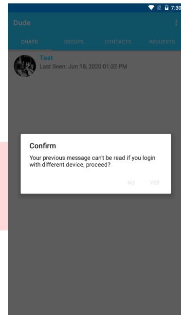
Gambar 4.11 Logout
