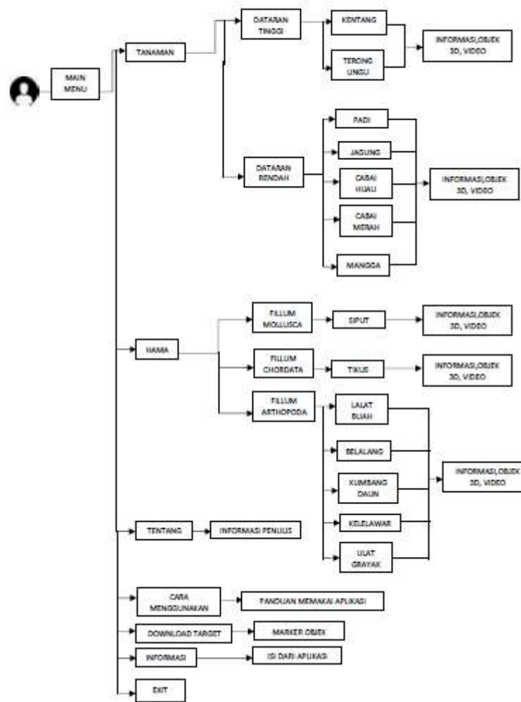
Gambar 4 Usecase Diagram
