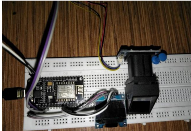
Gambar 3.5 Prototype Perangkat Keras Biometric Fingerprint Attendance.
