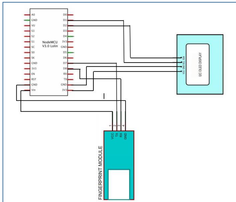
Gambar 3.4 Schematic Biometric Fingerprint Attendance
