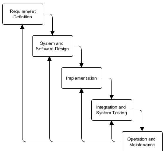
Gambar 2-1 SDLC Waterfall [1]
