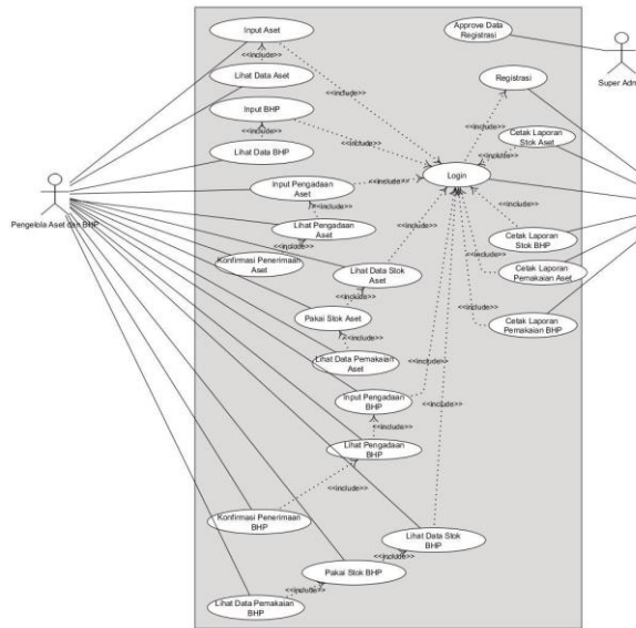
Gambar 3- 12 Use Case Diagram
