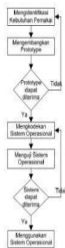
Gambar 3.1 Metode Prototype
