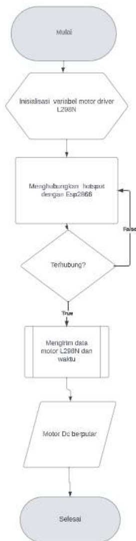
Gambar 3.2 Flowchart
