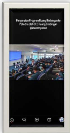
GAMBAR 4 Konten Collaboration
