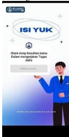
GAMBAR 5 Konten Connection
