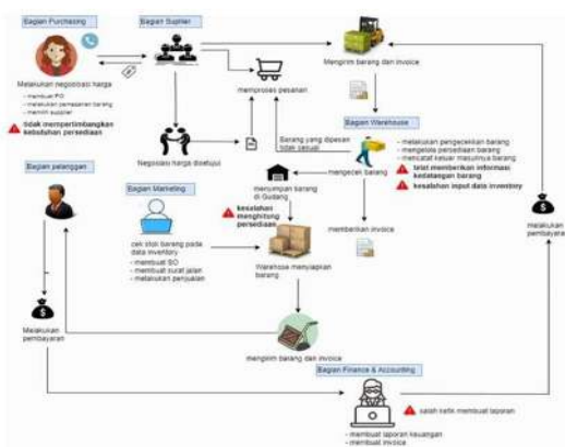
GAMBAR 1 Rich Picture
