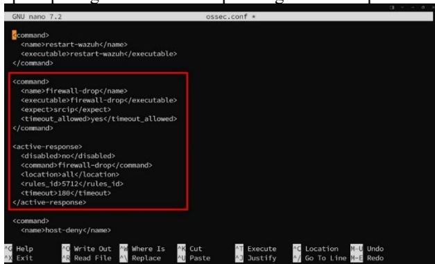
GAMBAR 10 Active respons brute force SSH
