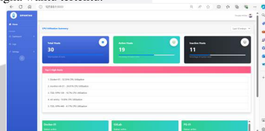
GAMBAR 3.1 Menu Home
