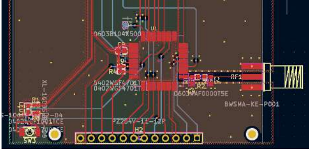
GAMBAR 14 Via Ground
