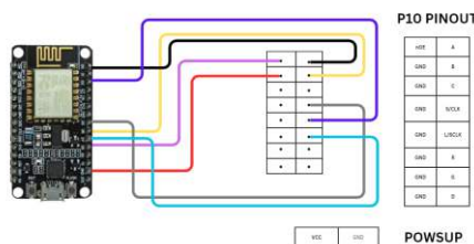
GAMBAR 8. Wiring ESP8266-LED Matriks
