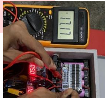
GAMBAR 13 Rangkaian Baterai 4S 2 paralel, 4 series
