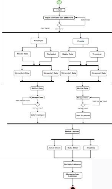
GAMBAR 4 Activity Diagram
