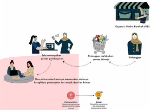
GAMBAR 1 Rich Picture
