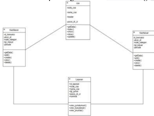
GAMBAR 5 Class Diagram
