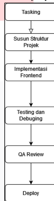
Gambar 4 Flowhart Waterfall
