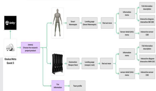
GAMBAR 4 (Blok Diagram Analisis)
