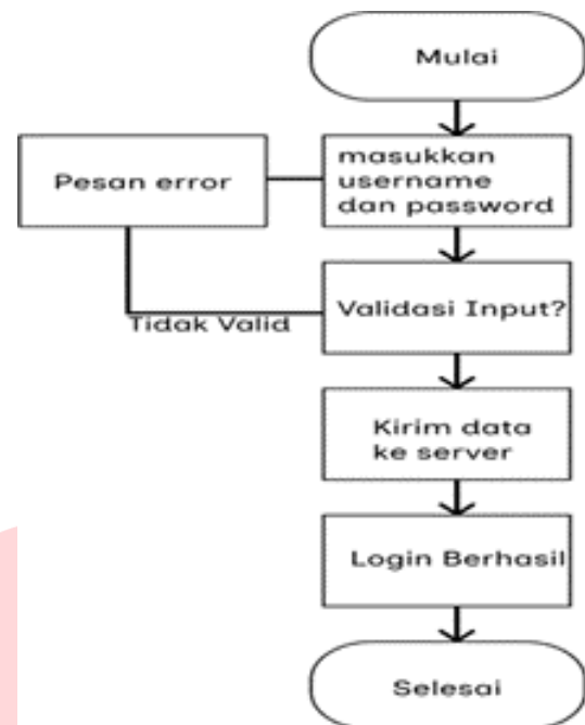
GAMBAR 2 Flowchart Login
