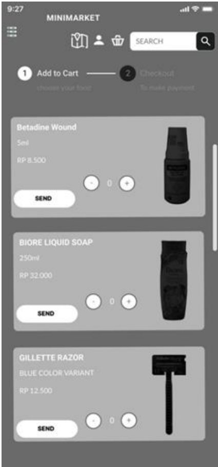
GAMBAR 10 Wireframe Minimarket
