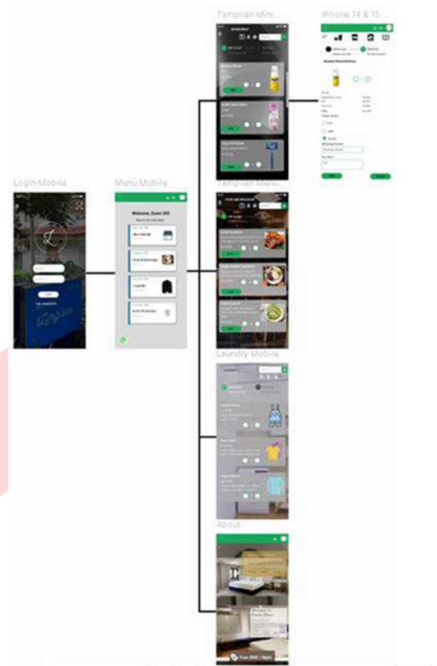
GAMBAR 22 Diagram Prototype
