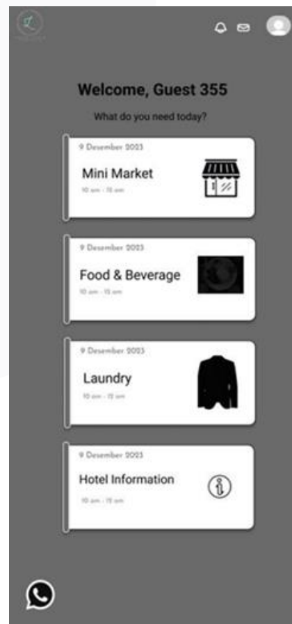
GAMBAR 9 Wireframe Dashboard
