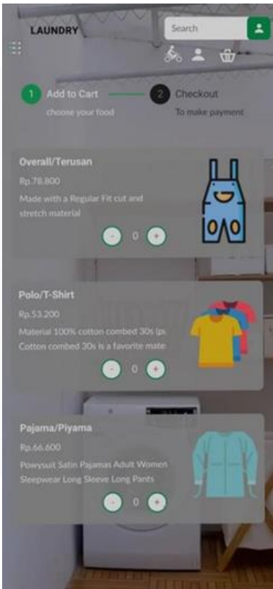
GAMBAR 19 Prototype Laundry
