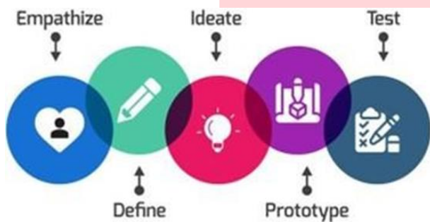
GAMBAR 3 Design Thinking
