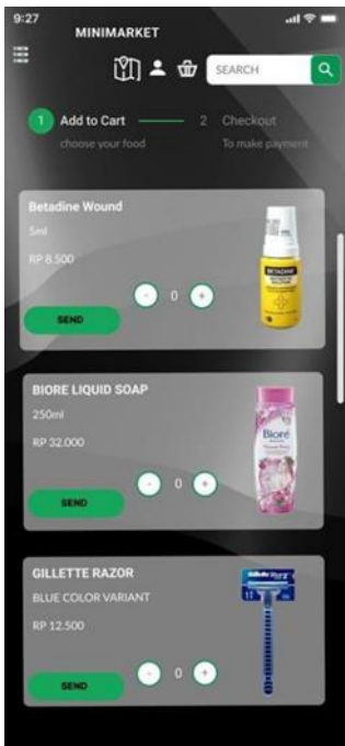
GAMBAR 17 Prototype Minimarket
