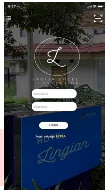
GAMBAR 15 Prototpye Login
