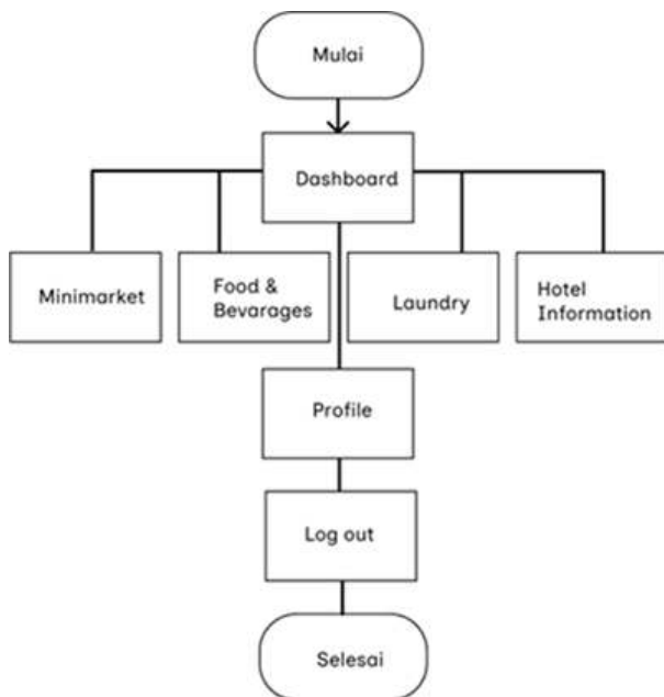
GAMBAR 4 Flowchart Fitur
