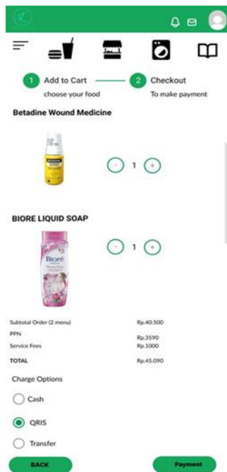
GAMBAR 20 Prototype Checkout
