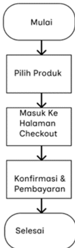
GAMBAR 5 Flowchart Checkout
