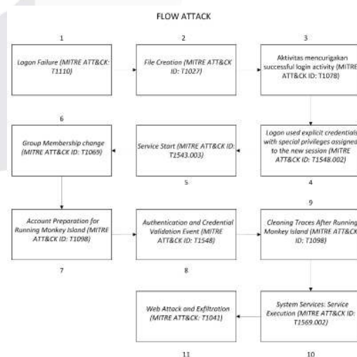
GAMBAR 2 Flow Attack
