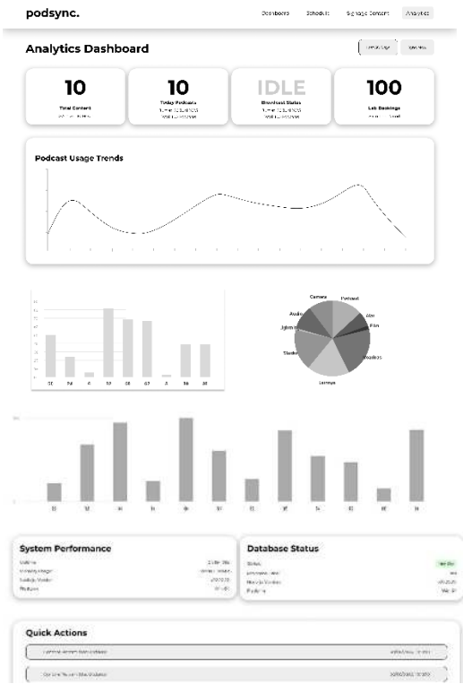
GAMBAR 8 Wireframe Analytics Page
