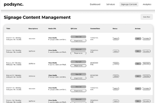
GAMBAR 7 Wireframe Content Management Page
