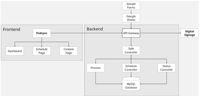
GAMBAR 3 Diagram Arsitektur Sistem "Podsync"
