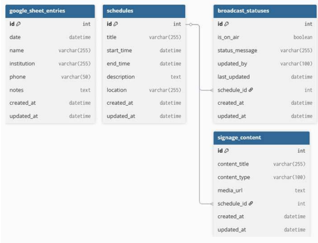
GAMBAR 4 ERD Database “Podsync”
