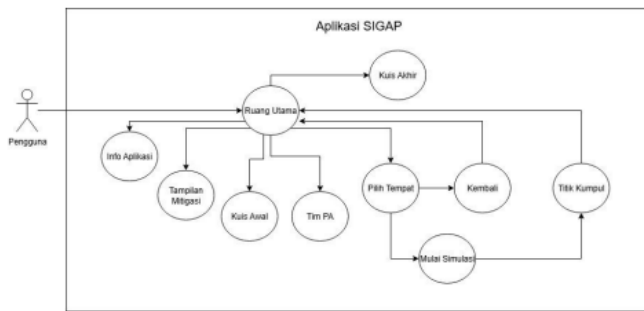
GAMBAR 2 Usecase Diagram
