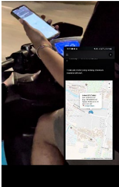
GAMBAR 7 Test Drive (1)
