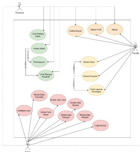
GAMBAR 2 Usecase Diagram
