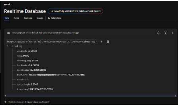
GAMBAR 6 Realtime Database Firebase GPS IoT Tracking
