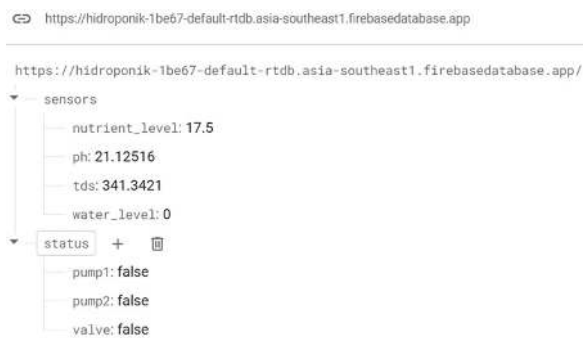
GAMBAR 4 Struktur Firebase Realtime Database
