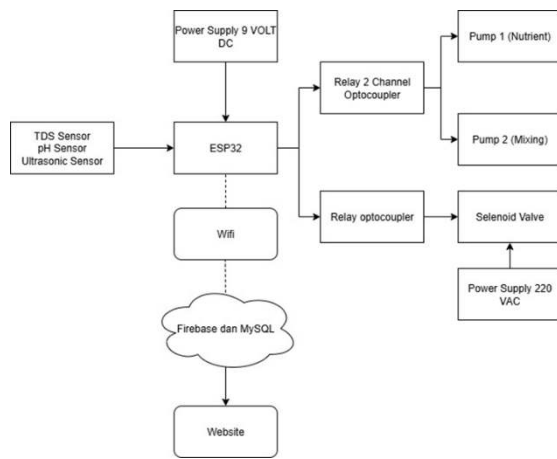
GAMBAR 6 Block Diagram Sistem
