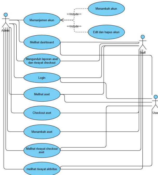
GAMBAR 2 Usecase Diagram
