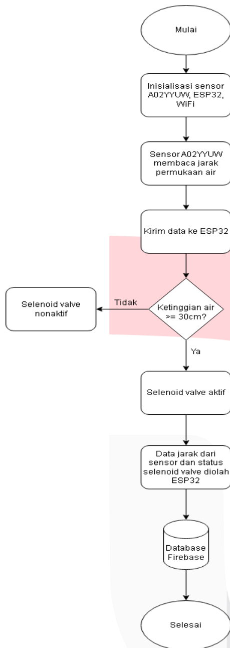
GAMBAR 3 Flowchart sistem
