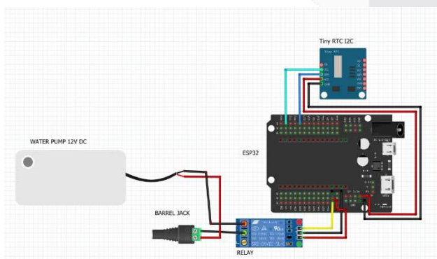
GAMBAR 7 Diagram Wiring
