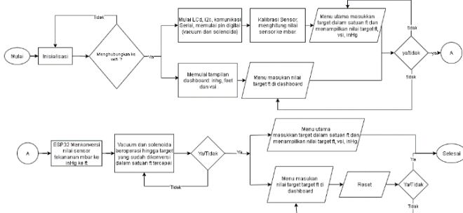
GAMBAR 2 Flowchart Sistem
