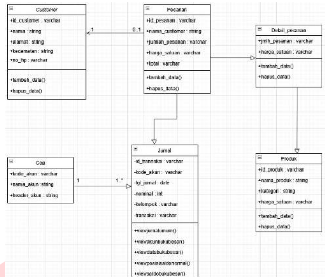
GAMBAR 4 Class Diagram
