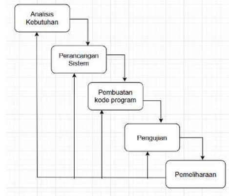
GAMBAR 1 Metode Waterfall
