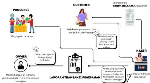
GAMBAR 2 Rich Picture
