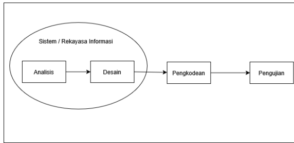
GAMBAR 1 Model Waterfall
