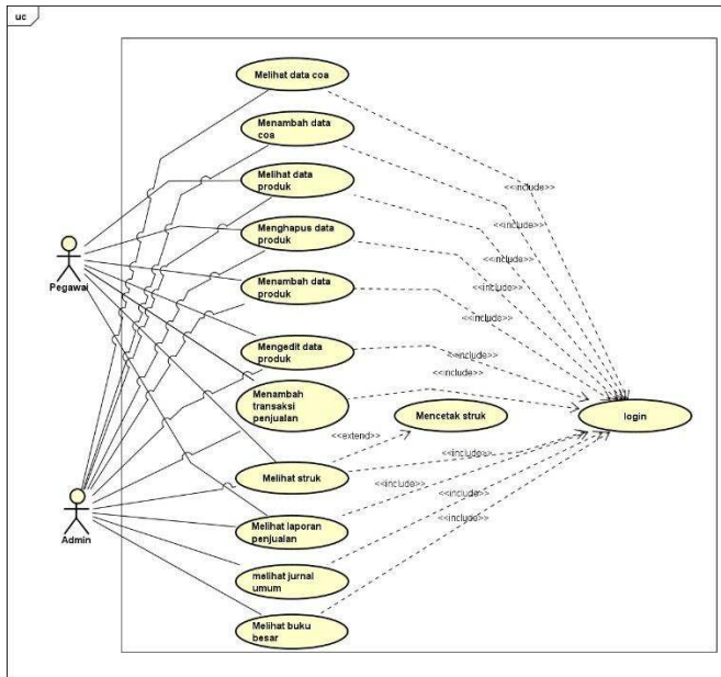
GAMBAR 4 Usecase Diagram
