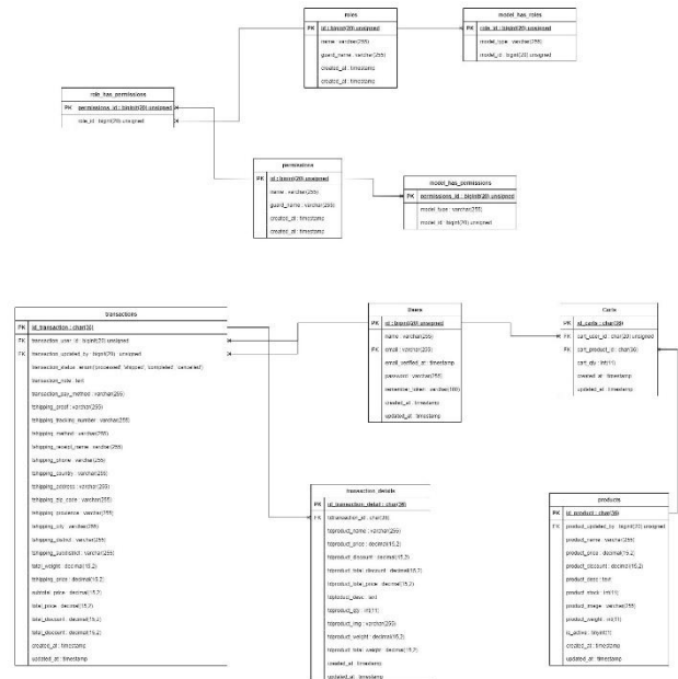
GAMBAR 3 Entity Relationship Diagram Toko Unyil
