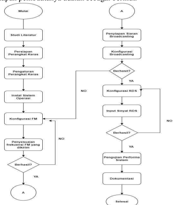
Gambar 3 Flowchart
