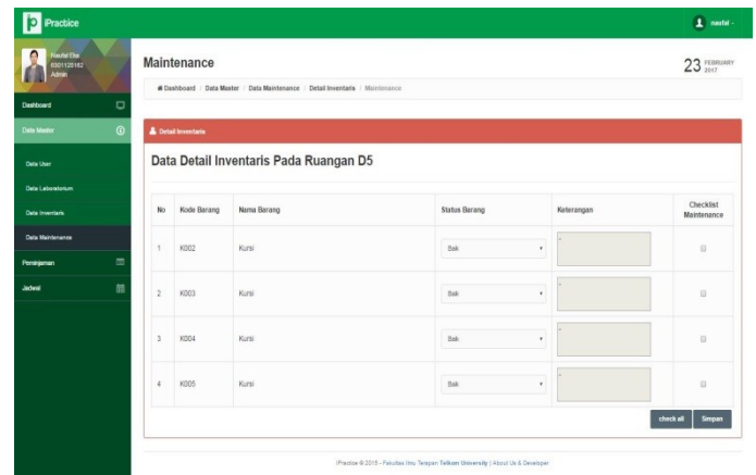
Gambar 19 Halaman Maintenance Inventaris
