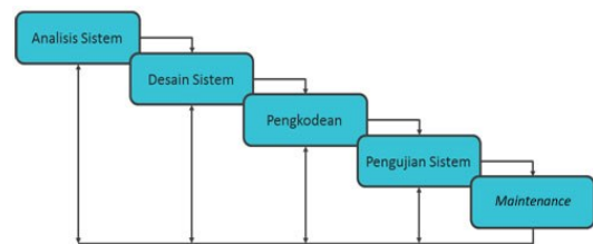
Gambar 1 Pendekatan Waterfall [1]
