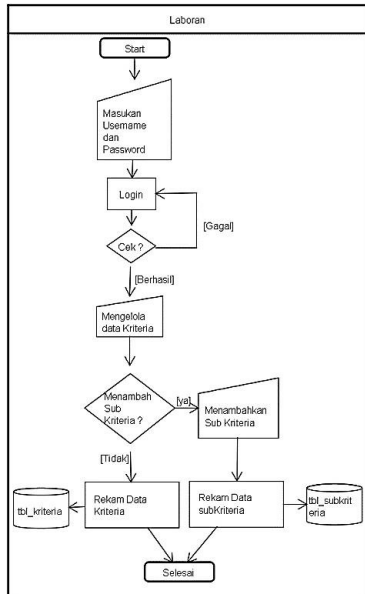
Gambar 6 Flowmap Usulan Data Kriteria
