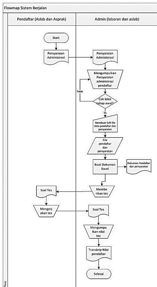
Gambar 1 Flowmap Sistem Berjalan
