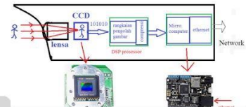
Gambar 2.8 Diagram Alur CCTV Network [2]
