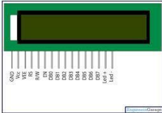
Gambar 2. Gambar PIN LCD
