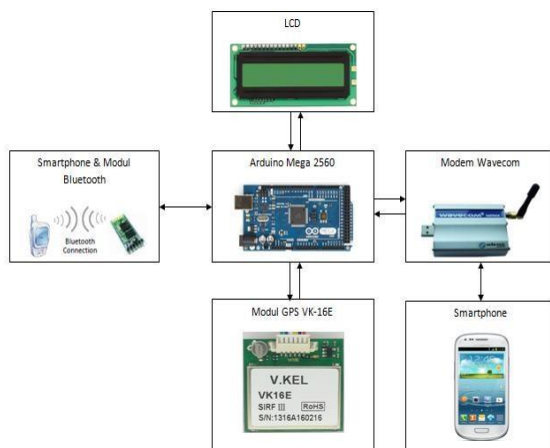
Gambar 8. Blok Diagram
