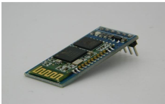
Gambar 3. Bluetooth HC-05
