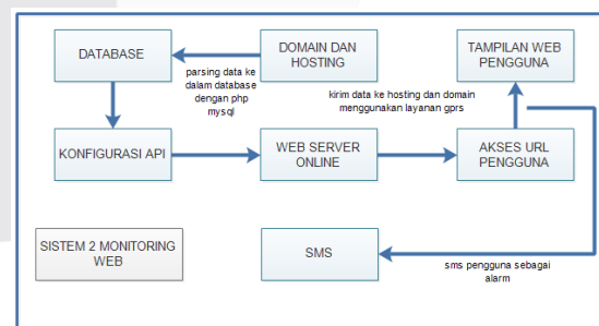
Gambar 3-2 Blok Diagram Sistem Monitoring
