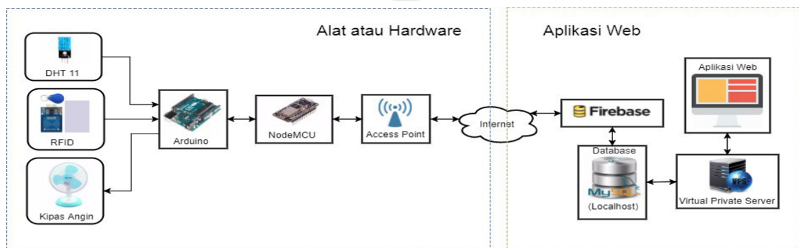
Gambar1 Sistem Monitoring Kinerja Kipas Angin
