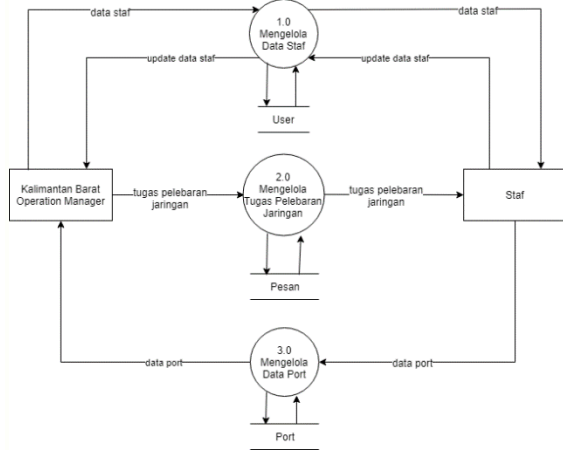
Gambar 3-6 Data Flow Diagram level 0
