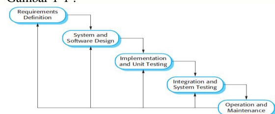
Gambar 1-1 Model Waterfall
