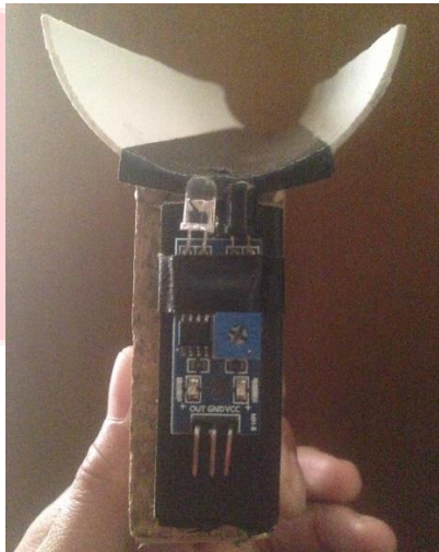
Gambar 4.3 Sensor Infrared
