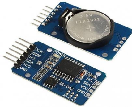
Gambar 2.3 RTC [7]
