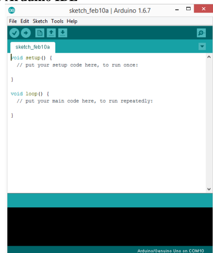
Gambar 2.5 Arduino IDE [9]
