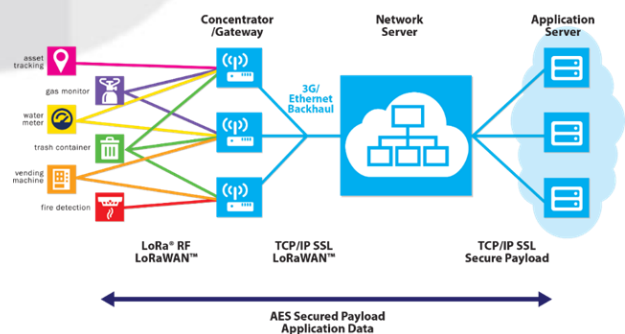
Gambar 2.1 Diagram Jaringan Lora
