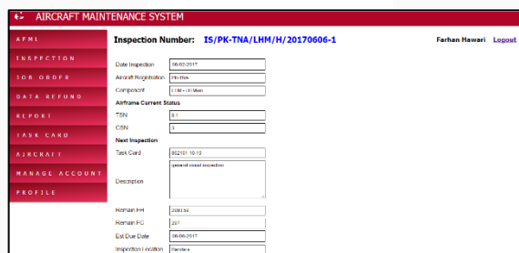
Gambar 6 Tampilan Input Inspection Schedule
