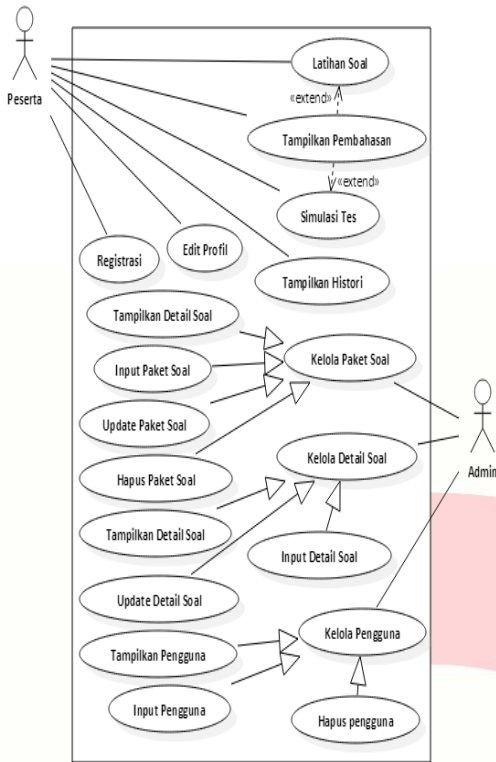
Gambar 3-4 Use Case
