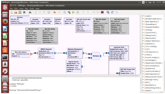
Gambar 4.4-1 NFM.grc
