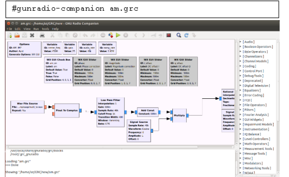
Gambar 4.3-2 File AM.grc
