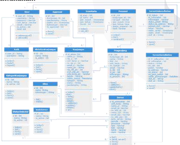
GAMBAR 4 CLASS DIAGRAM
